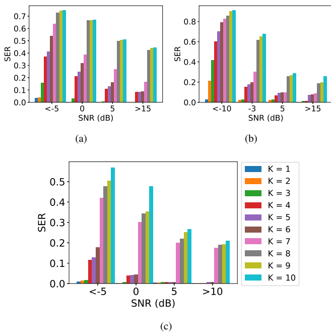
Fig. 13: SER for Super-LoRa for various superposition orders and (a) SF = 7 , (b) SF = 8 , and (c) SF = 9 .
