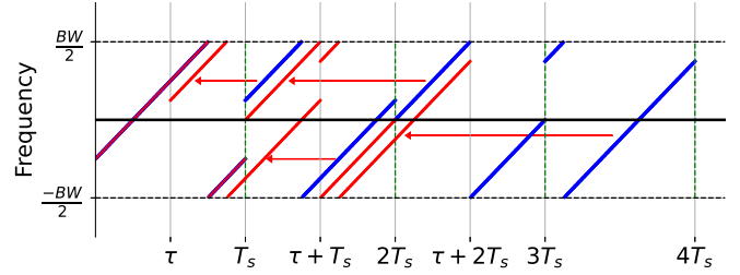
Fig. 3: Illustration of LoRa superimposed payload symbols with superposition order K = 2 and \tau = \frac{T_s}{2} . In blue, four consecutive symbols transmitted over 4T_s transmission time. In red, Super-LoRa transmits the same four symbols over 2T_s + \tau transmission period ( \frac{T_s}{2} overlap between consecutive symbols), showing great potential of throughput improvement.
