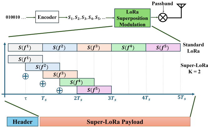
Fig. 4: Illustration of Super-LoRa payload superposition compared to standard LoRa. Super-LoRa superimposes several payload symbols without introducing an extra overhead on the packet structure (utilize the same header as standard LoRa). In this example, Super-LoRa utilizes K = 2 with \tau = \frac{T_s}{K} .
