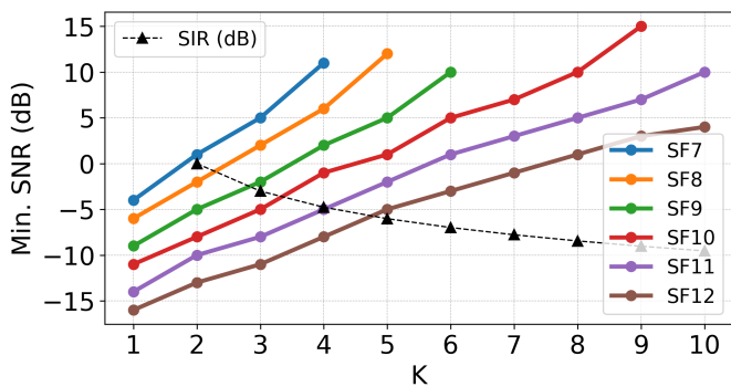
Fig. 8: Minimum required SNR to achieve SER = 10^{-1} for each superposition order K . Note that there is a penalty of around 4-5 dB for each additional K symbols superimposed. In black, we plot at the same figure the resulting SIR (defined as SIR = \frac{1}{K-1} ) for each superposition order K .
