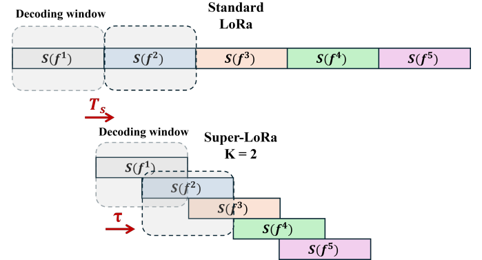
Fig. 7: Illustration of Super-LoRa decoding window compared to standard LoRa. The receiver aligns the decoding window with the first payload symbol, which is detected through the preamble as performed in standard LoRa. Instead of decoding each payload symbol every chirp time T_s , the receiver in Super-LoRa decodes every \tau seconds. This maintains the same processing capabilities while offering higher resource utilization.
