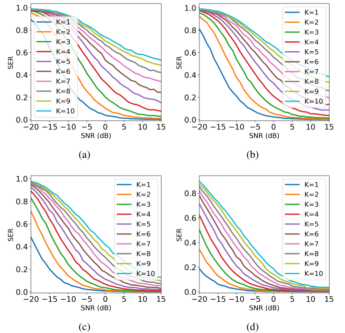
Fig. 9: SER for Super-LoRa over Rayleigh fading channel with various Superposition orders and (a) SF = 7 , (b) SF = 8 , (c) SF = 10 , and (d) SF = 12 .
