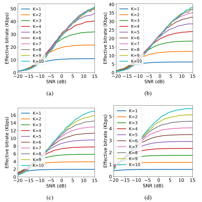
Fig. 11: Effective bitrate calculated based on Equ. (21) for Super-LoRa for various superposition orders and (a) SF = 7, (b) SF = 8, (c) SF = 10, and (d) SF = 12.
