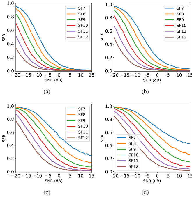
Fig. 10: SER for Super-LoRa over Rayleigh fading channel with various SF and (a) K = 2 , (b) K = 3 , (c) K = 6 , and (d) K = 8 .
