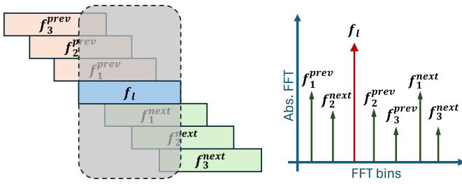
Fig. 5: Once the receiver aligns the decoding window with the first payload symbol, all subsequent chirps will follow sequentially, with sliding the decoding window at a multiple of time delay \tau . The l^{th} payload symbol exhibits interference from K - 1 payloads to be decoded next, as well as K - 1 decoded earlier. In this example, the superposition order is K = 4 , with 2 \times (4 - 1) = 6 interfered peaks seen on the spectrum. The peaks of the interfered symbols are proportional to the time overlap with the target symbol.
